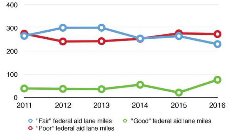
Presque Isle County, Michigan Road Condition of Federal Aid Lane Miles All County Roads
